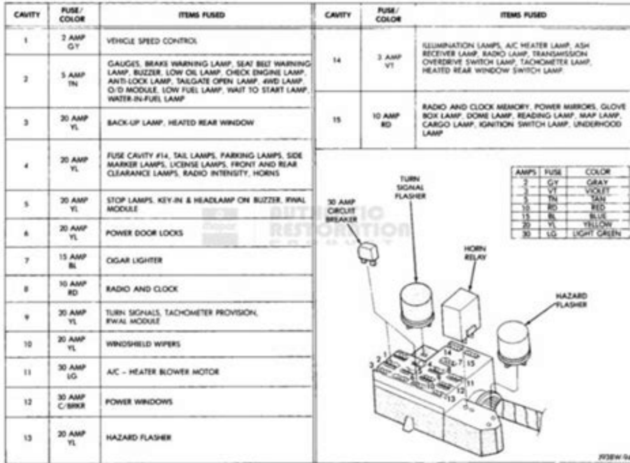
Fig. 12 Fuse Block and Relay Bank
